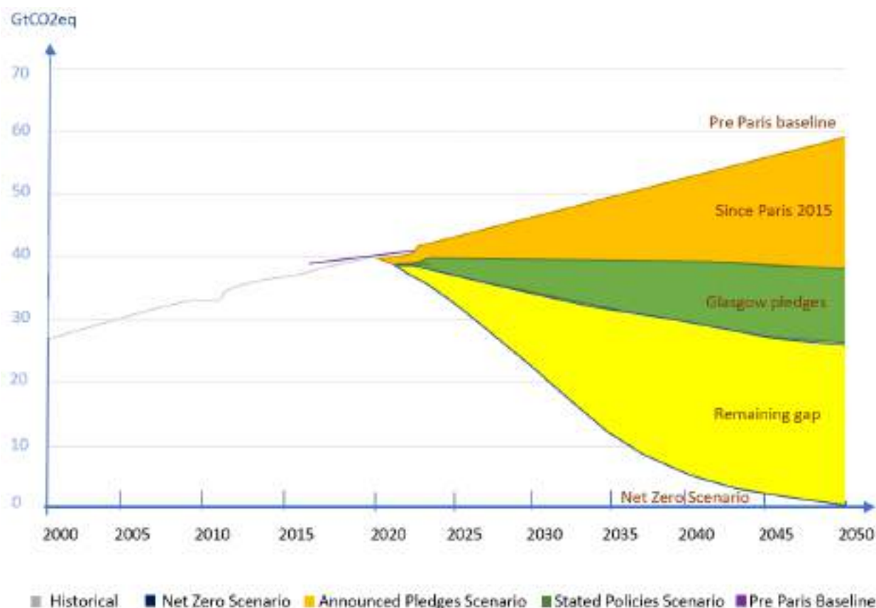
Figure 1. Global emissions by scenario, 2020–2050.
