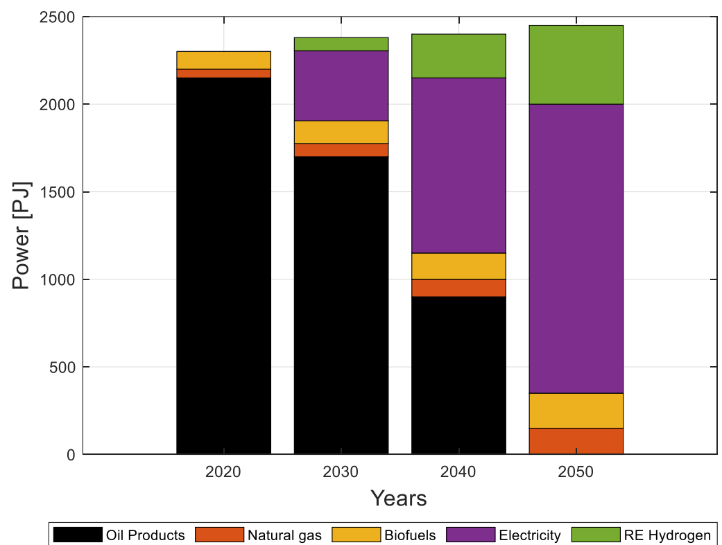
Figure 12. Interaction in the Mexican energy mix. Increased renewable energy and reduced fuel in the long term for transportation.
