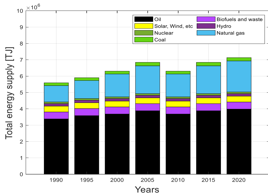
Figure 4. Historical total energy supply (TES) by source in Mexico, inspired from [80].
