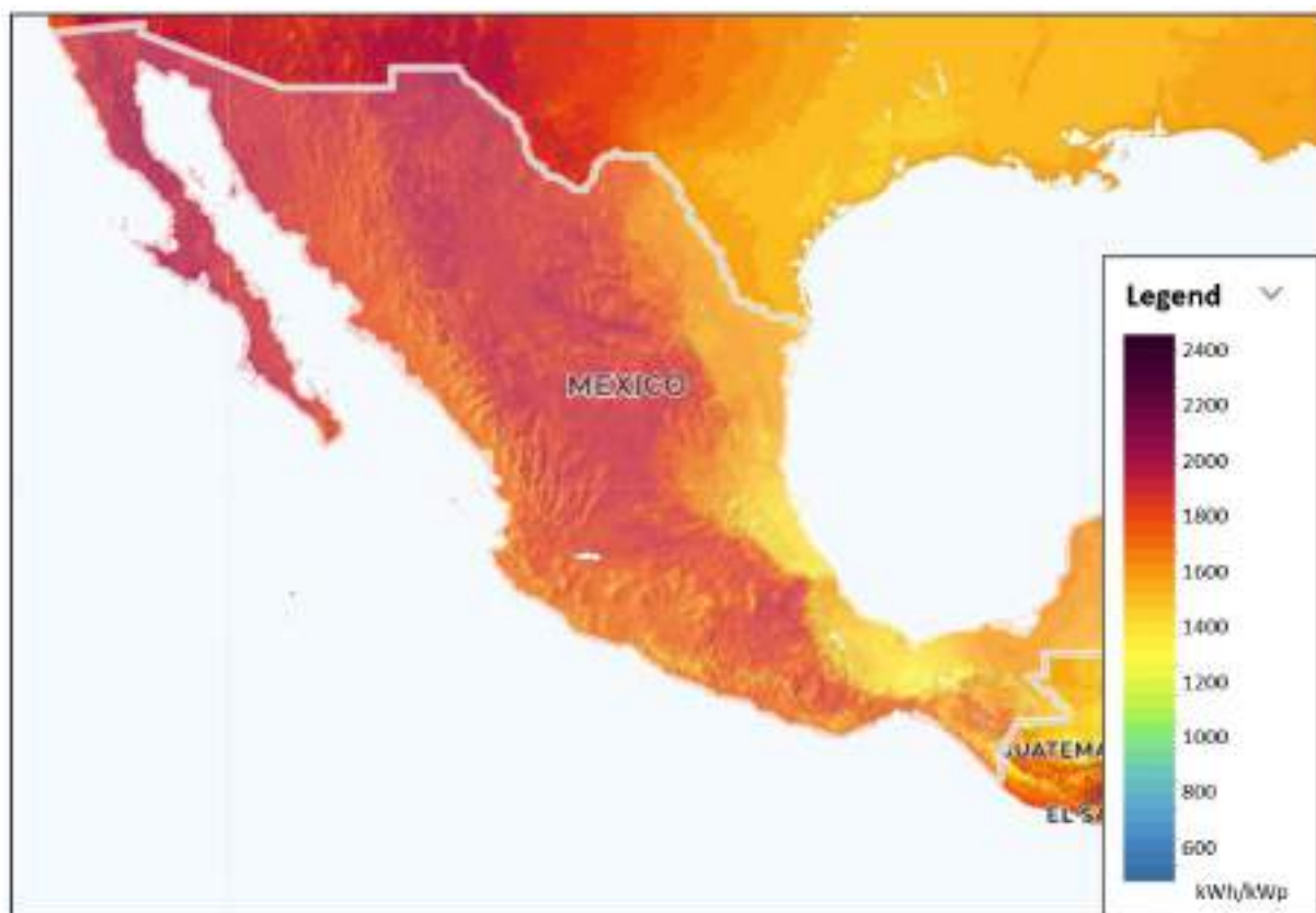
Figure 7. Solar photovoltaic power potential in Mexico, analyzed by the authors in free software Global Solar Atlas [93].
