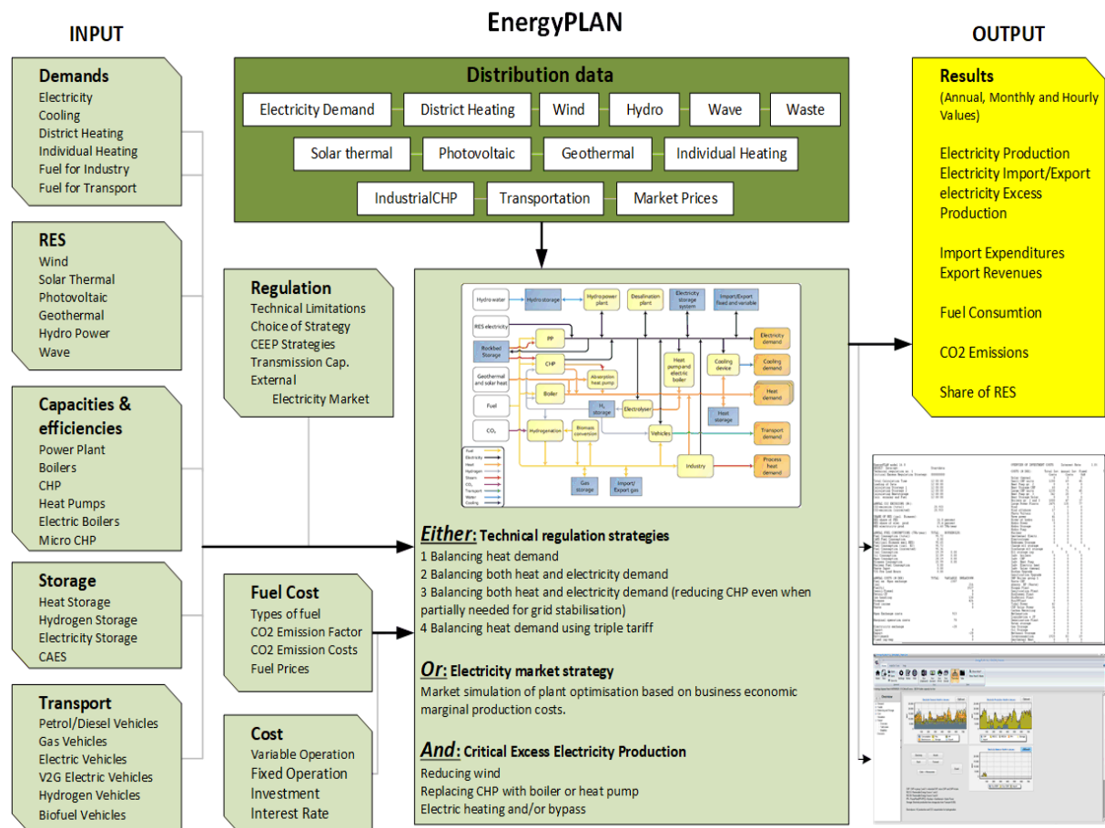
Figure 3. Analysis model for smart energy planning, EnergyPLAN V16.2. Model inspired in [77].
