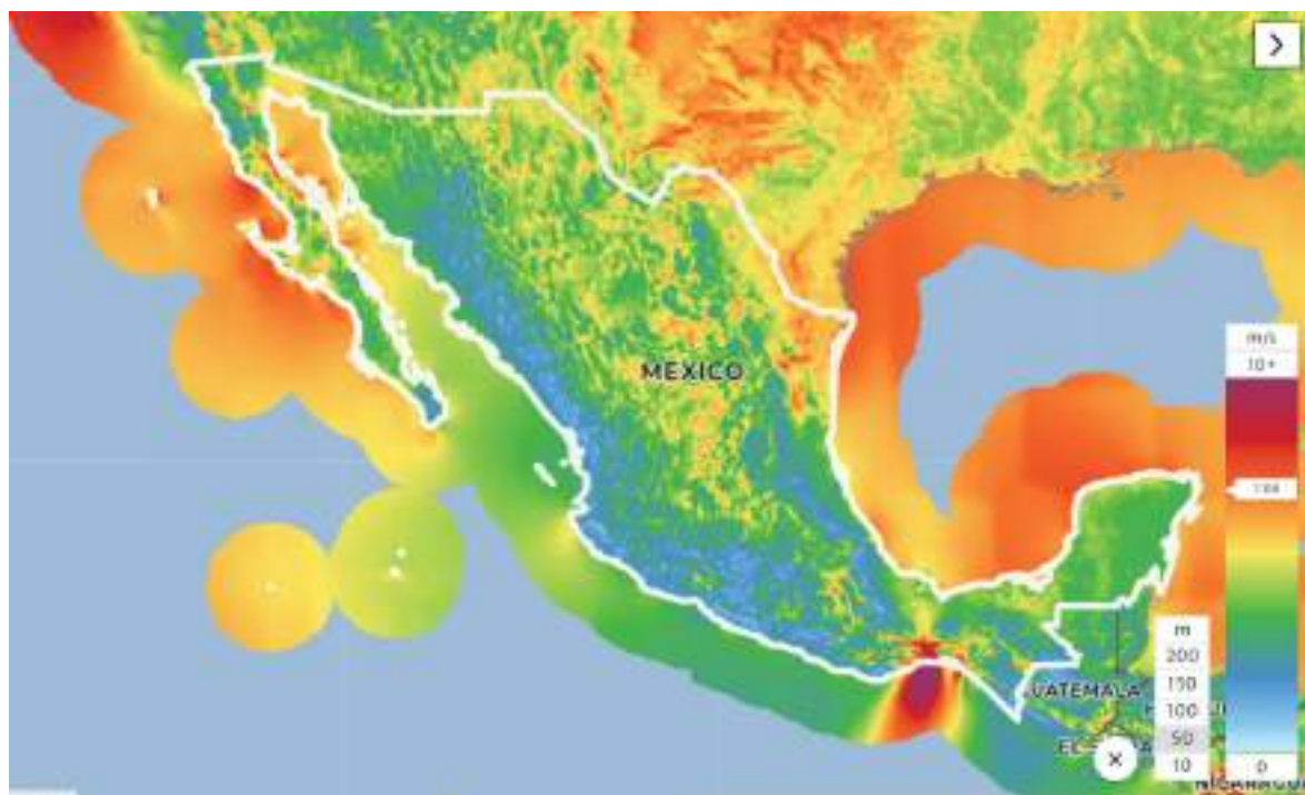
Figure 8. Wind power potential in Mexico, analyzed by the authors in free software Global Wind Atlas [96].
