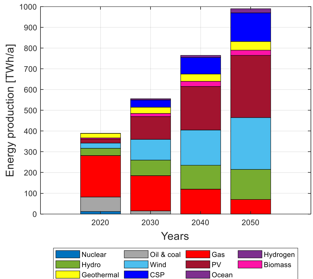
Figure 11. Power production in Mexico for 2050.
