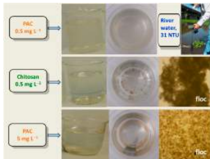
Figure 9. Turbidity reduction in water samples from the Culiacán River using chitosan and commercial poly(aluminum chloride) (PAC). Images were captured using a digital camera and a light microscope (magnification 10×) after flocculation trials. The images were taken in the Environmental Laboratory of the Faculty of Engineering Culiacán-UAS, Mexico, by Diana V. Félix-Alcalá.
