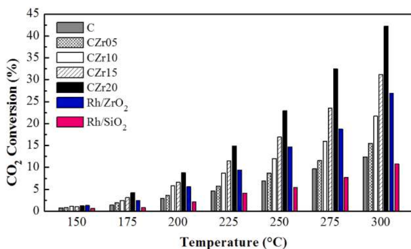
Fig. 6. Steady-state CO 2 conversion over Rh-supported catalysts. GHSV= 15,000 h -1 , H 2 :CO 2 =4:1.
