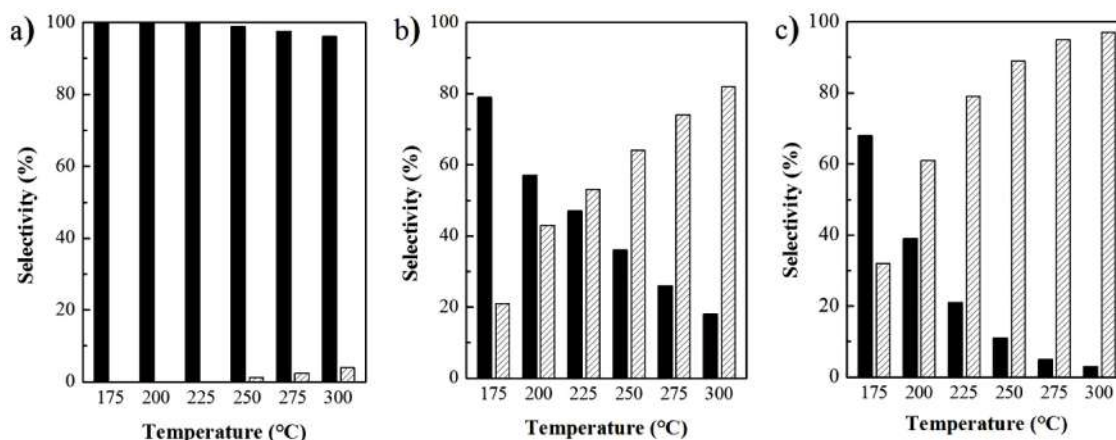
Fig. 7. Selectivity towards CH 4 and CO of the representative samples (CO; CH 4 ). a) C; b) CZr10; CZr20.
