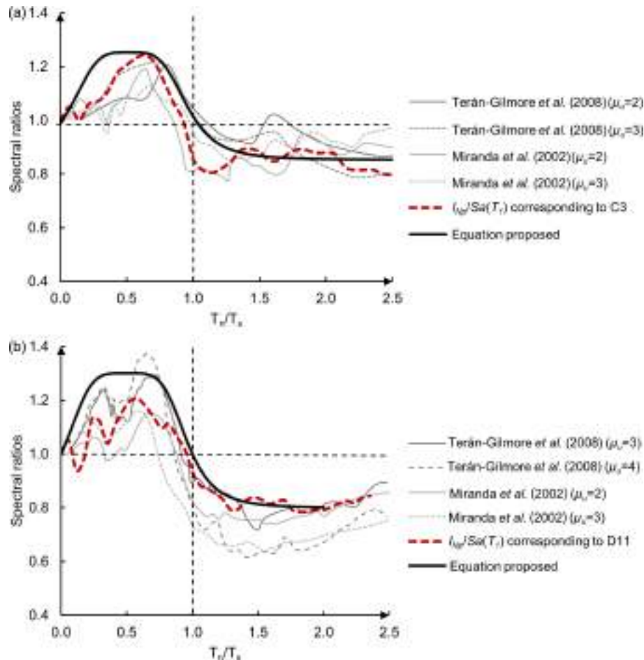
Figure 10. Mean ratios of strength demands of degrading and of non-degrading systems corresponding to (a) firm ground (zone C) and (b) soft soil (zone D) of Mexico City.
