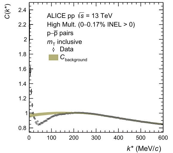
Fig. 1. Measured p-\bar{p} correlation function (empty points) with statistical (line) and systematic (grey boxes) uncertainties. The band represents the C_{\text{background}}(k^*) fit as described in the text.
