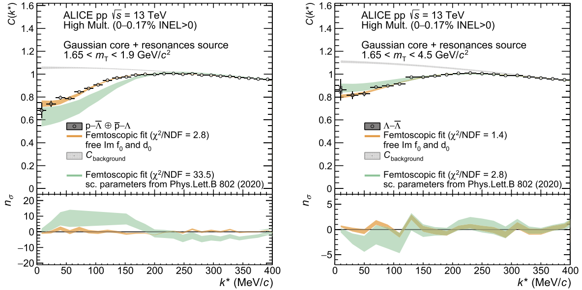
Fig. 3. Measured correlation function of p\text{-}\bar{\Lambda} (left) and \Lambda\text{-}\bar{\Lambda} (right) pairs for two representative m_T bins. Statistical (bars) and systematic (boxes) uncertainties are shown separately. Results using the Lednický-Lyuboshits formula with Pb-Pb scattering parameters [23] are shown in light green. Orange bands are the results with d_0 and \mathcal{I}f_0 as free parameters. In grey the corresponding C_{\text{background}}(k^*) , multiplied by the normalization constant N_D , is shown. The reported average \chi^2/\text{NDF} is evaluated in the k^* interval [0, 400] MeV/c and it includes correlations between the data points. Lower panel: same as in Fig. 2.
