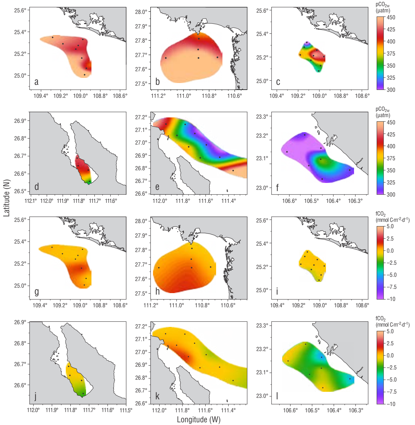
Figure 4. Horizontal distribution of seawater CO 2 partial pressure ( p\text{CO}_{2w} ) and CO 2 flux variability ( f\text{CO}_2 ) for the different subregions: NAV2016 (a, g), GUA2016 (b, h), NAV2017 (c, i), BC2017 (d, j), MUL2017 (e, k), and MAZ2017 (f, l). The figures were confectioned using Ocean Data View.
