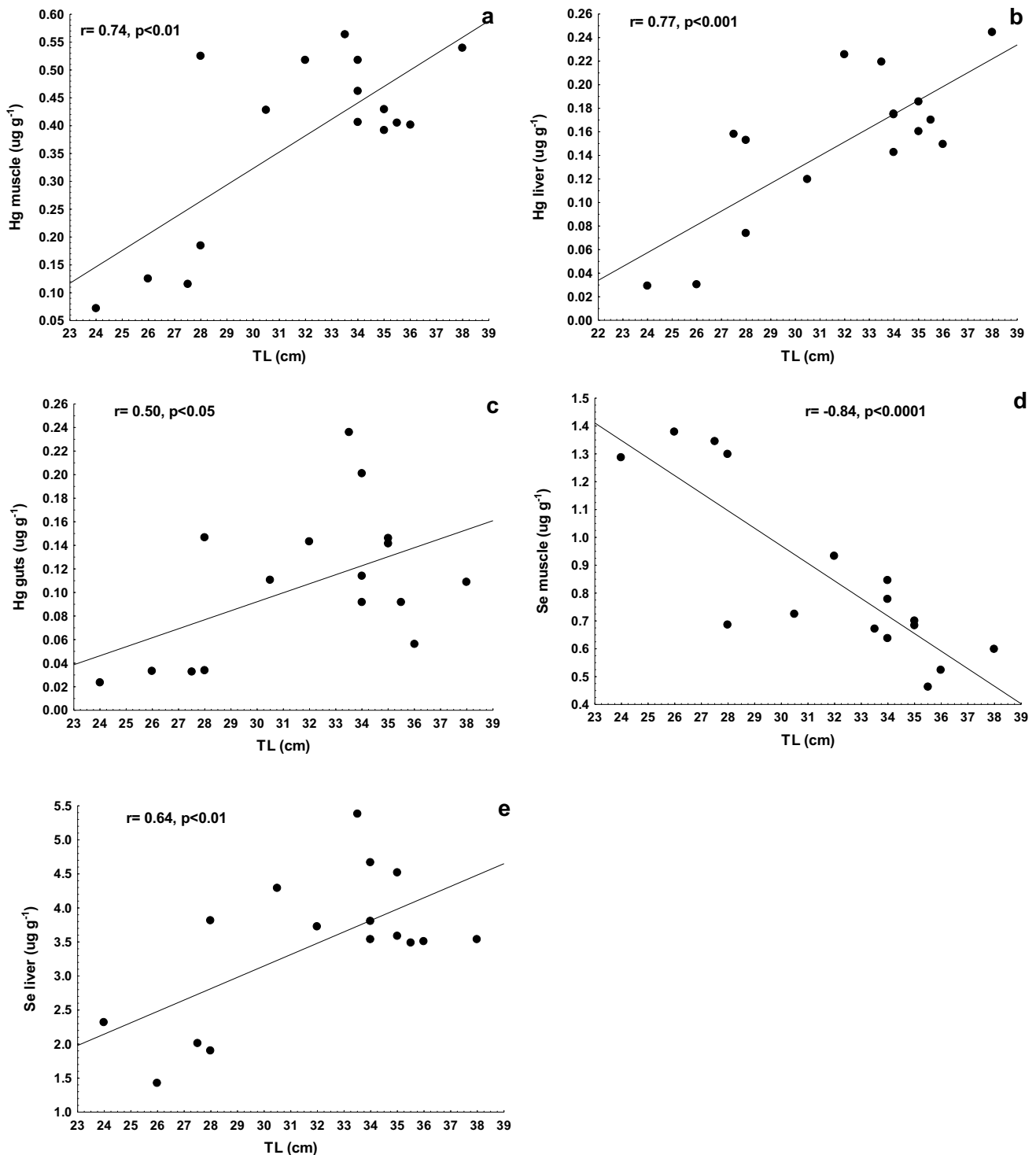
Fig. 3 Variation of the concentration of Hg in muscle (a), liver (b), and guts (c) with length (TL), as well as Se in muscle (d) and liver (e) with the size of the largemouth bass
