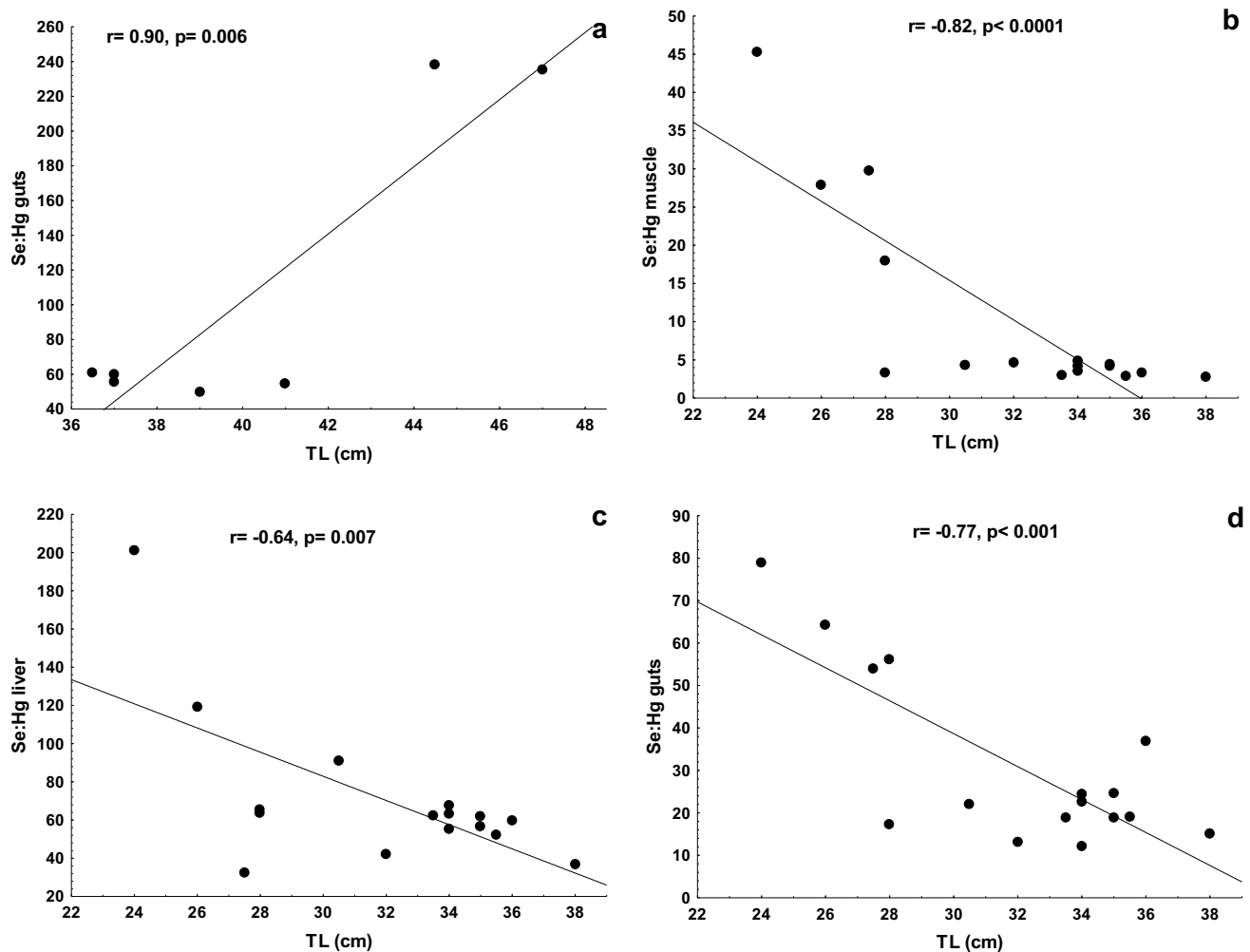
Fig. 2 Variation of Se/Hg molar ratios with length (TL) in guts of the carp (a), and muscle (b), liver (c), and guts (d) of the largemouth bass
