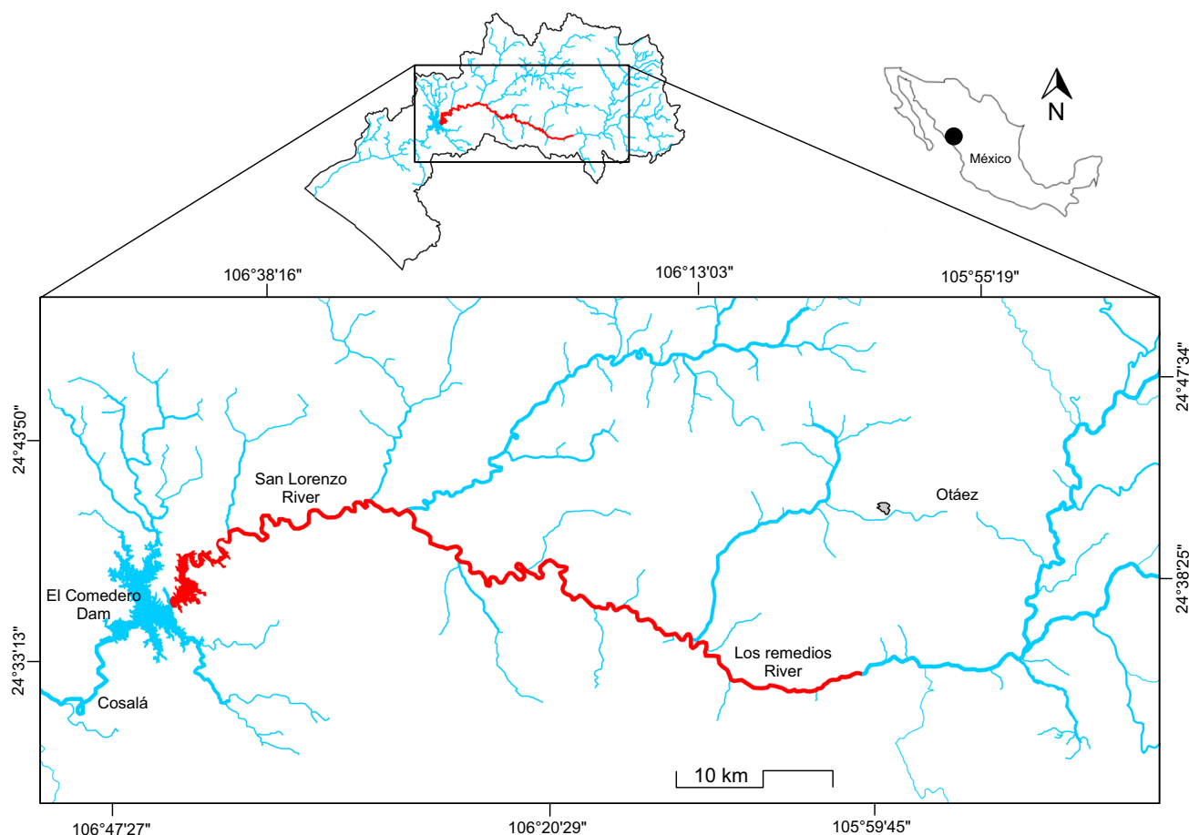
Fig. 1 Illustration of the spill-affected zone along Los Remedios River-San Lorenzo River (red); the right extreme corresponds to the discharge site where the mine-tailings dam failure occurred
