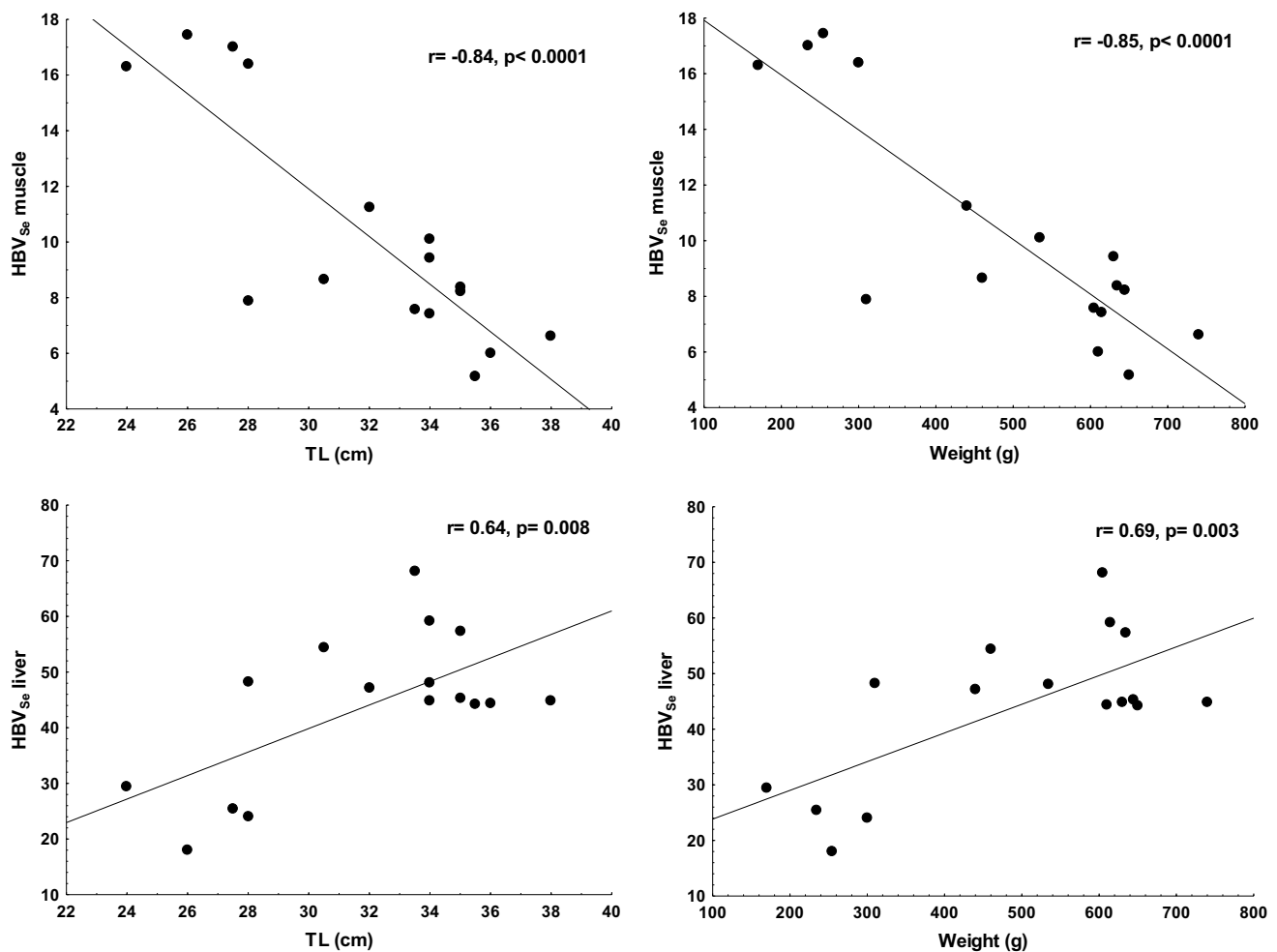
Fig. 4 Variation of HBV Se in– the muscle and liver with length and weight of the largemouth bass
