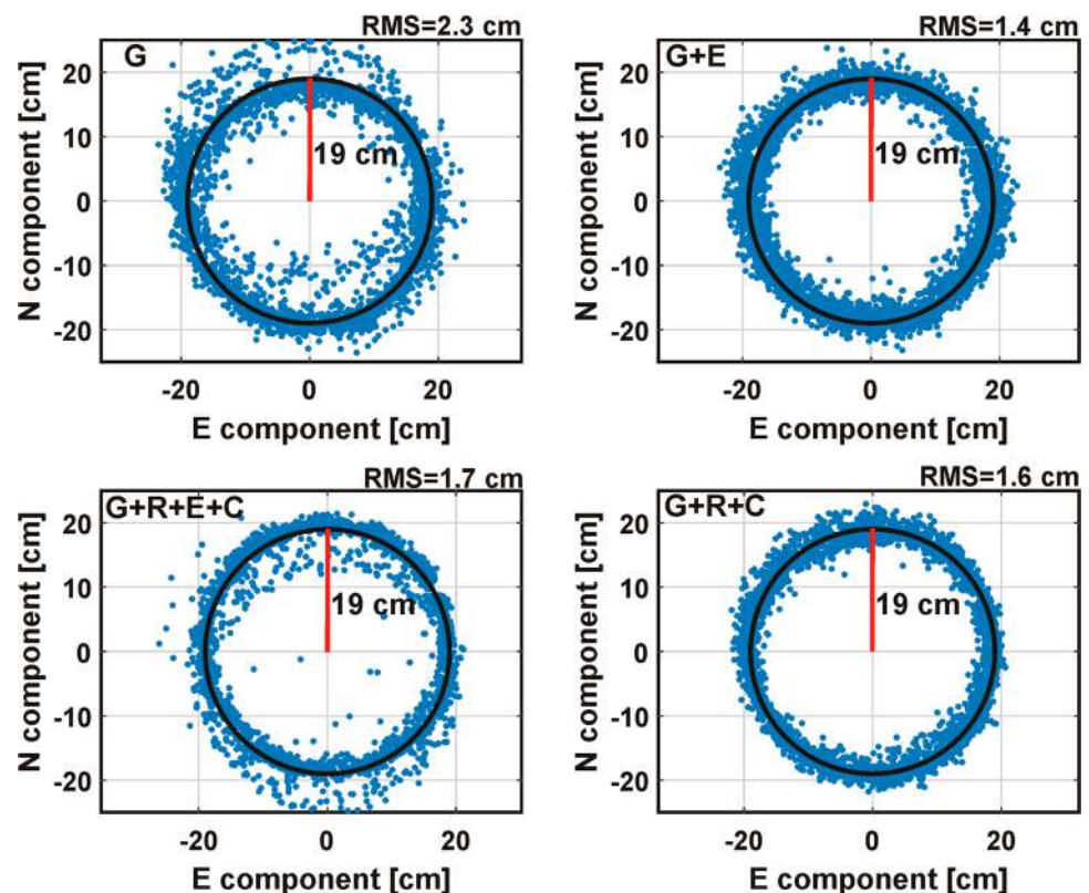
Fig. 10 Circular trajectory tracking of kinematic results obtained from various GNSS combinations. The blue dots represent the kinematic solutions of the Xiaomi Mi 8, and the black circle represent the reference circular movement
