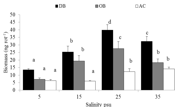
Figure 2. Dry organic biomass, organic biomass (OB) and ash content (AC) for Proales similis reared at different salinities (Mean±SD). Different letters indicate significant differences ( P<0.05 ) within salinities.
