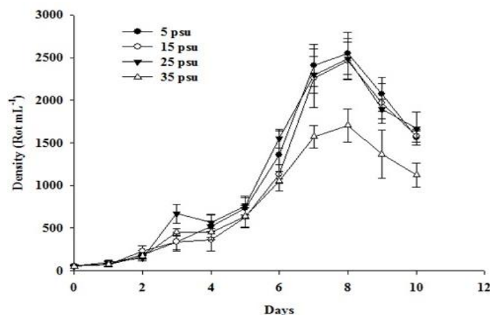
Figure 1. Population growth curves for P. similis reared at different salinities. Symbols indicate mean density \pm SD for a 10 day culture period. Some SD are not distinguishable due to small values.
