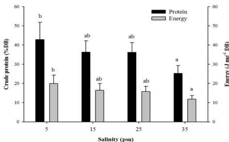
Figure 3. Crude protein and energy content relative to dry biomass (DB) for P. similis reared at different salinities. Different letters indicate significant differences ( P<0.05 ) at each salinity per variable.
