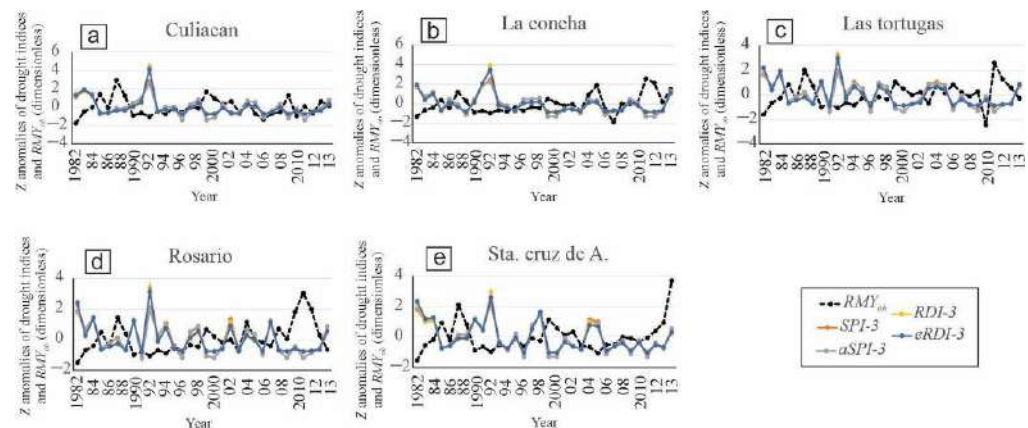
Figure 3. Z anomalies of the drought indices SPI-3 , aSPI-3 , RDI-3 and eRDI-3 , and RMY_{ob} (dimensionless). The black line refers to RMY_{ob} and the four meteorological drought indices in Sinaloa are shown in red ( SPI-3 ), gray ( aSPI-3 ), yellow ( RDI-3 ) and blue ( eRDI-3 ) (a–e).
