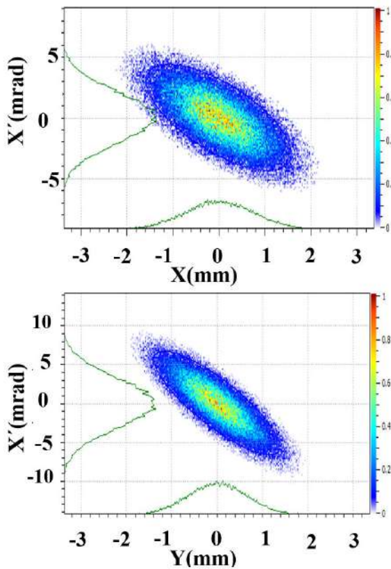
FIGURE 6. Transverse beam phase space at the end of the 60 MeV transport line before been injected in to the RF cavity for acceleration.
