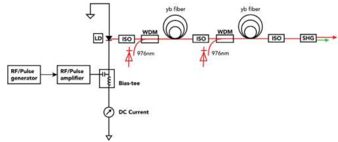
FIG. 4. Schematic of the rf-pulsed green-light driver laser system (LD, laser diode; ISO, optical isolator; WDM, wavelength division multiplexer; SHG, second harmonic generation crystal).
