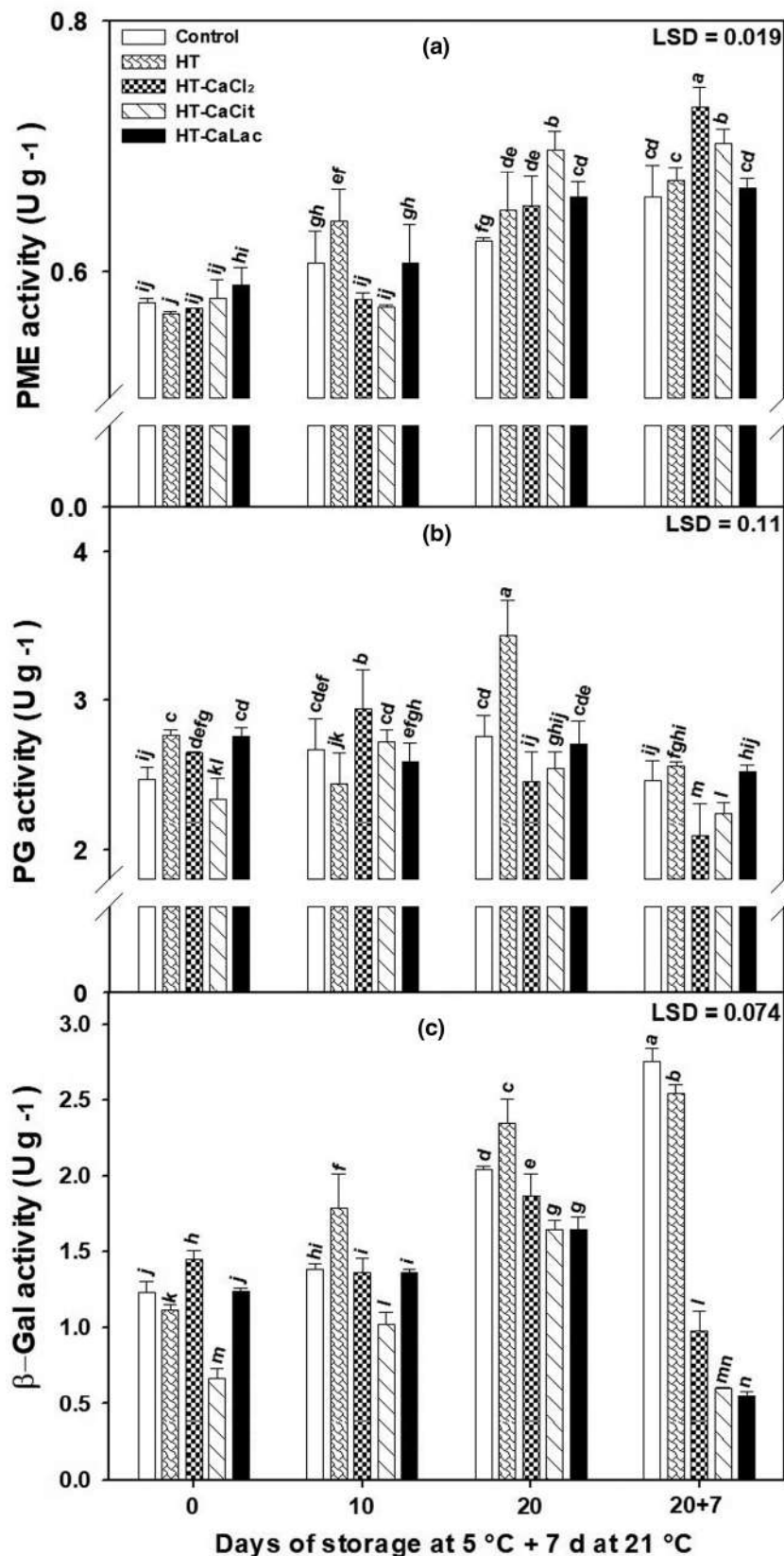
FIGURE 4 Pectin methylesterase (a), polygalacturonase (b), and \beta -galactosidase (c) activities in mango fruit treated with a hot water treatment (HT) and hot water treatment combined with calcium chloride (HT-CaCl 2 ), calcium citrate (HT-CaCit), or calcium lactate (HT-CaLac) and stored for 20 days at 5°C plus 7 days at 21°C. vertical bars on columns represent the standard deviation of the means of three replicates. Different letters indicate significant differences according to the Fisher's least significance difference (LSD) test.
